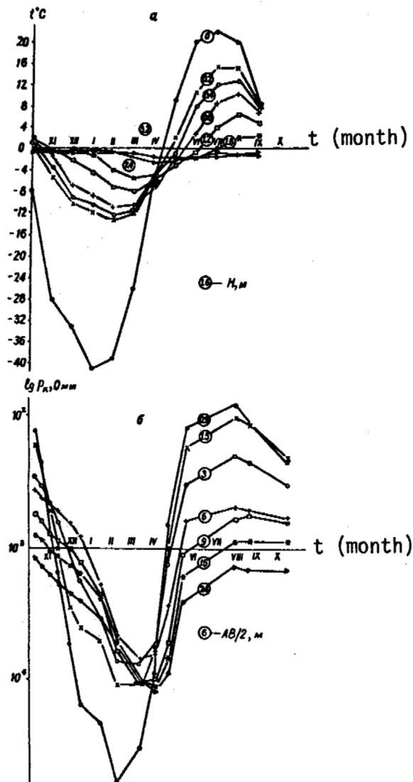
Temperature change and \rho_b , measured by the Vanner arrangement, in the yearly cycle (base, town of Yakutsk).
